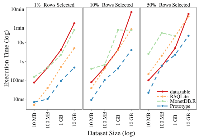
(b) Selection and Projection
