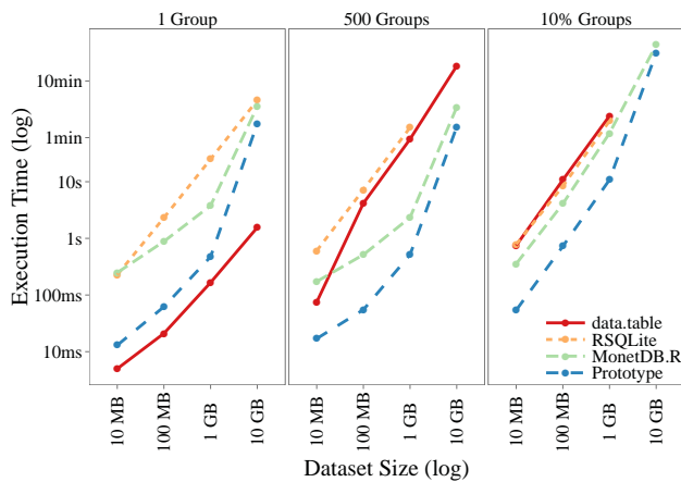
(c) Grouping and Aggregation
