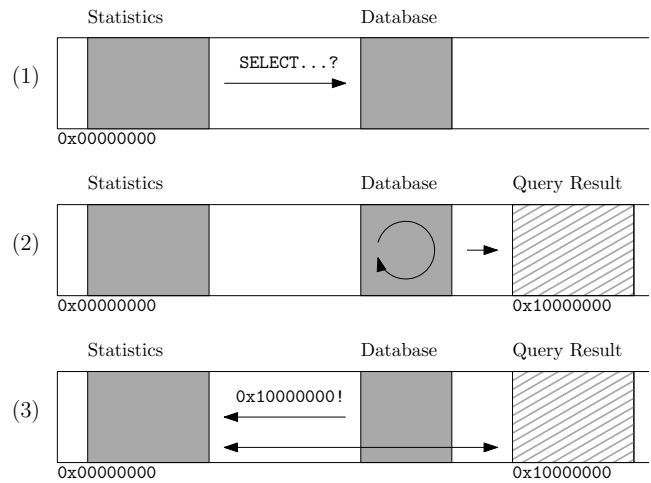
Figure 1: Communication Flow within Process Space
